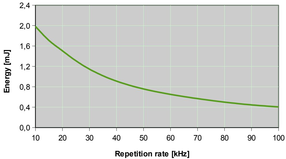
Sol 40W 1064nm: Pulse Energy
