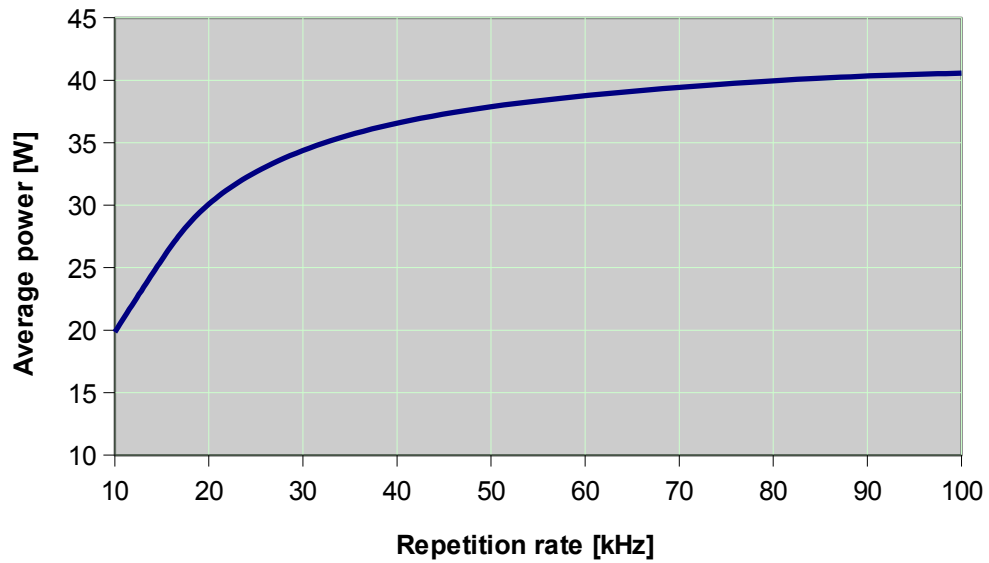
Sol 40W 1064nm: Average Power
