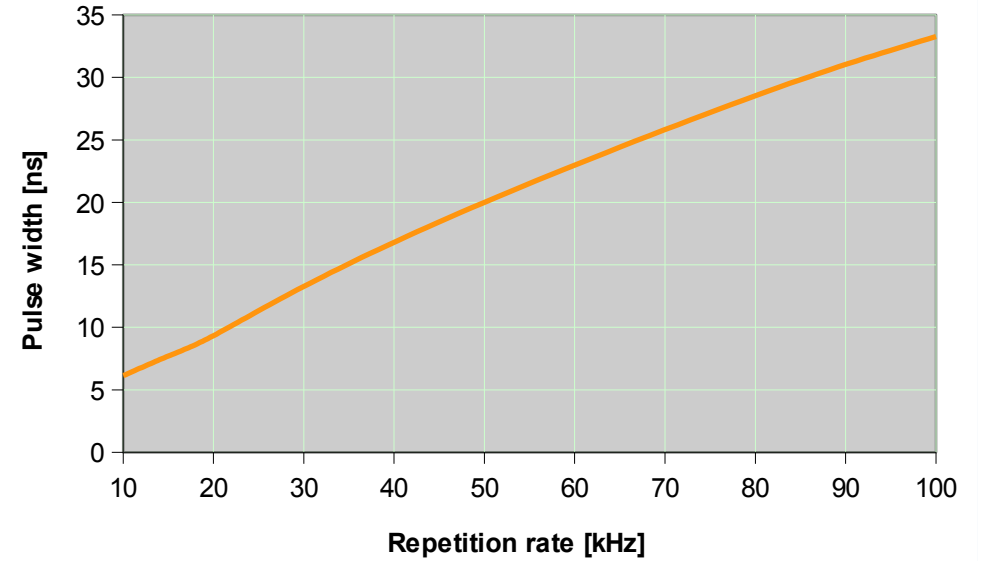
Sol 40W 1064nm: Pulse Width
