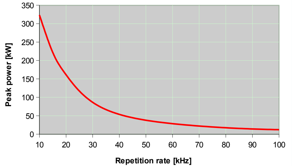
Sol 40W 1064nm: Peak Power
